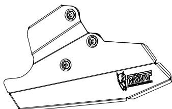
COPERTURA IN ALLUMINIO / ALUMINIUM COVER 50.CR.011.0 + KIT
